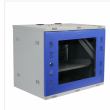
S-R 12U 610X550X400 MM 1U CANTILEVER TRAY 255 MMD X 1 6 SOCKET PDU, MOUNTING HARDWARE, FAN
