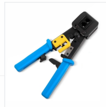
CRIMPING TOOL PASS TROUGH (S-CT PASS TROUGH)
